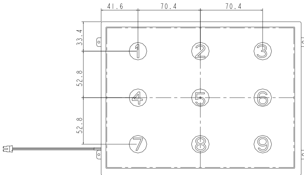
Fig8-1 Measuring point
